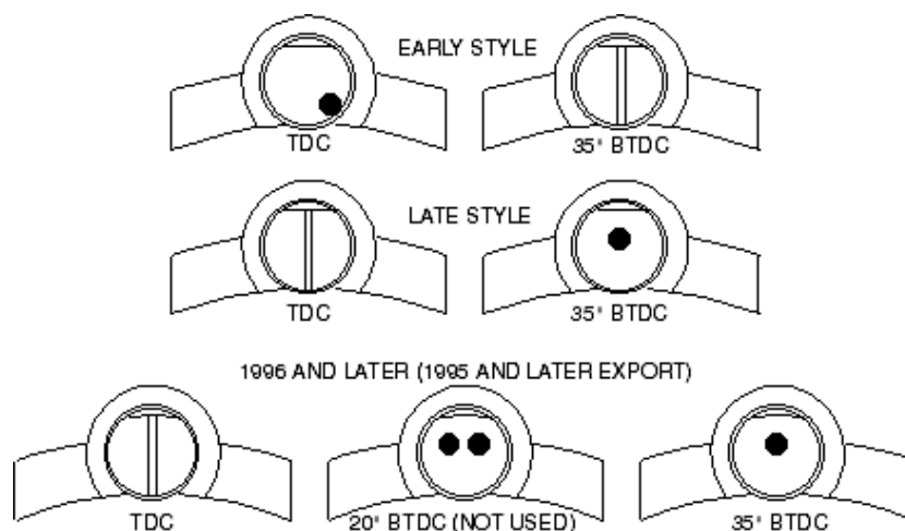
Figure 8 - Front Cylinder Timing Marks
