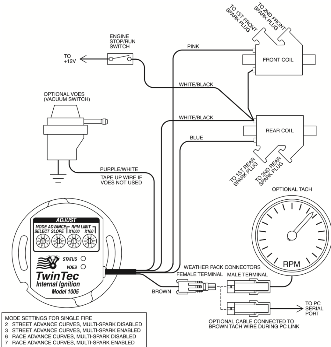
Figure 1 – Model 1005/1005S Dual Spark Plug Wiring Diagram
