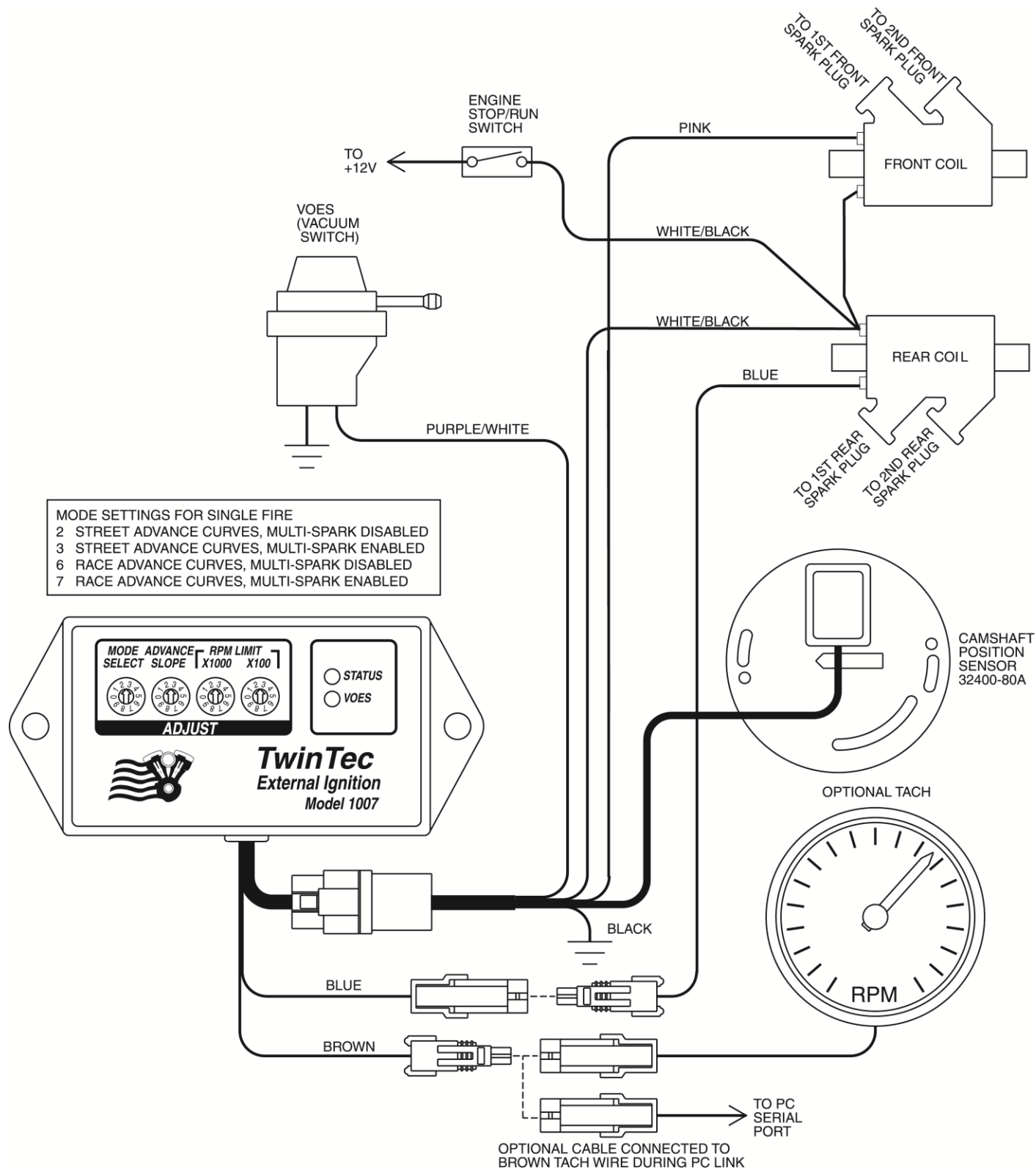
Figure 2 – Model 1006/1007 Dual Spark Plug Wiring Diagram
